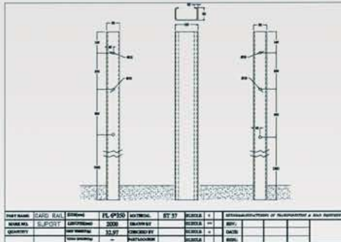
Support (Post)
