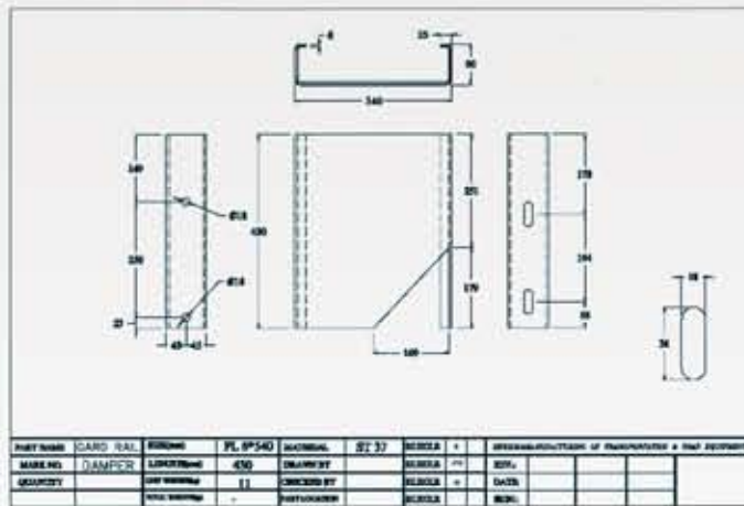
Damper (Spacer)
